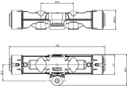
OVERALL DIMENSIONS W/ CSA M6
